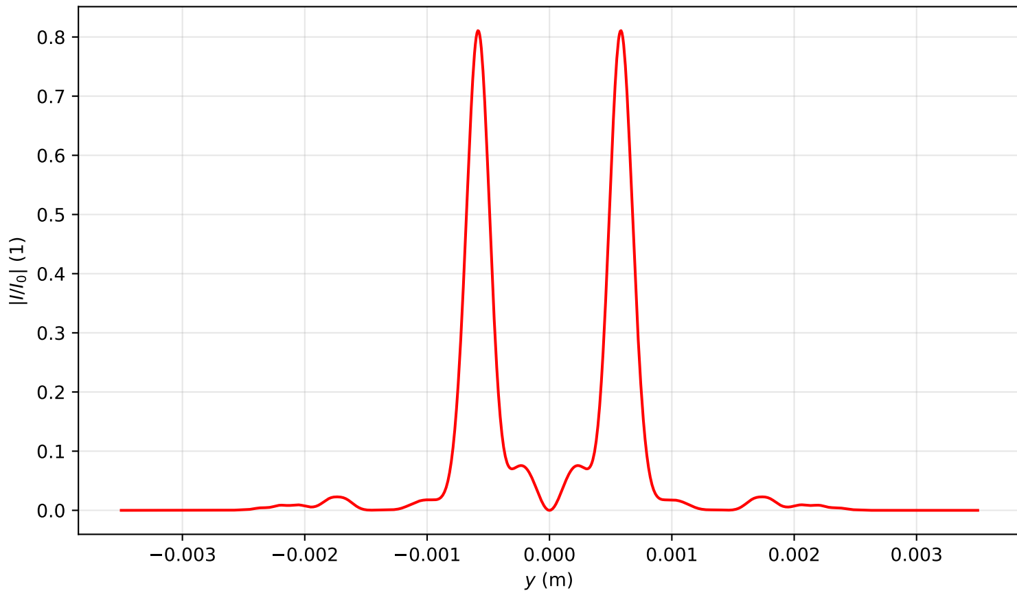
Intensity profile I(x=0, y, z=1.513)/I_0 , P_{in}=9.0P_{cr} , artificial time
